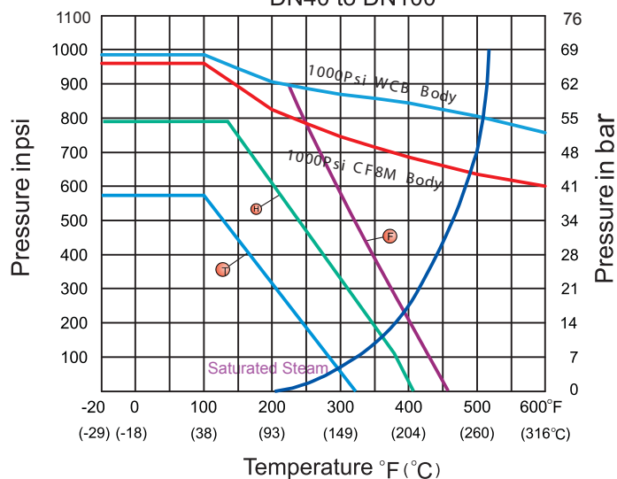
Full Bore : NPS 1 ½ ~ NPS 4 DN40 to DN100
